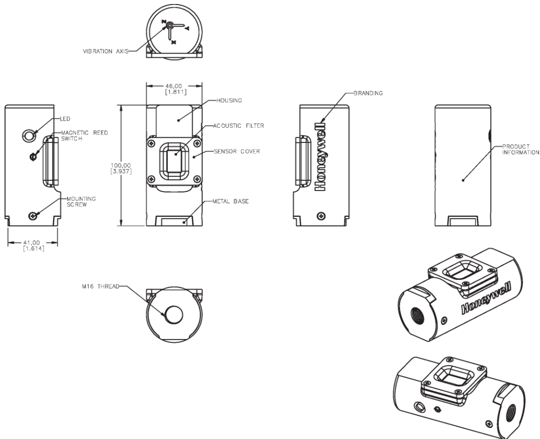
Figure 3– Physical Dimensions
