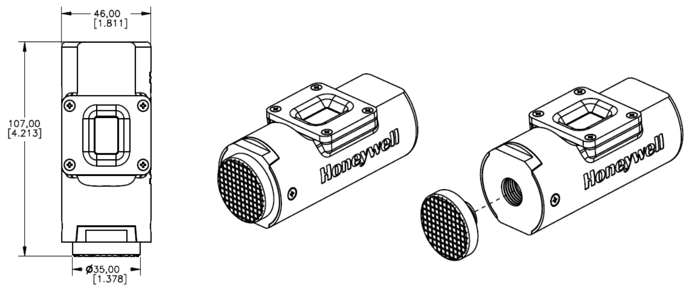
Figure 8 – Epoxy mount
