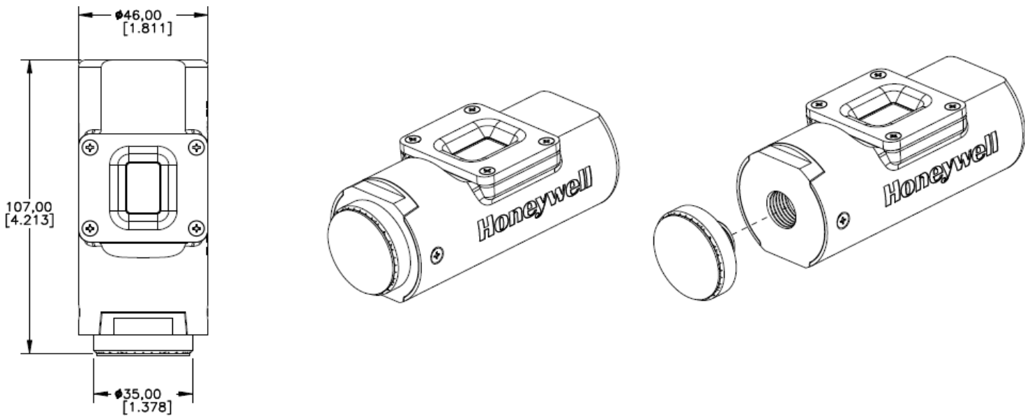
Figure 5– Adhesive mount
