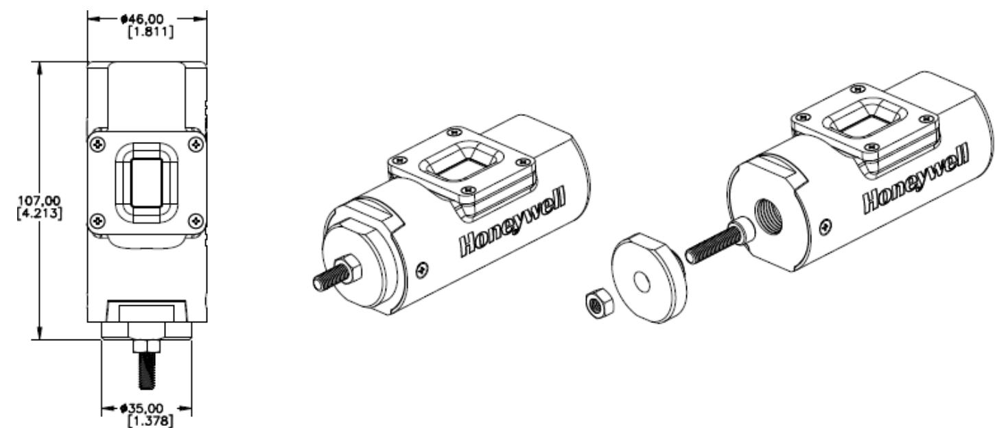
Figure 7 – Screw mount
