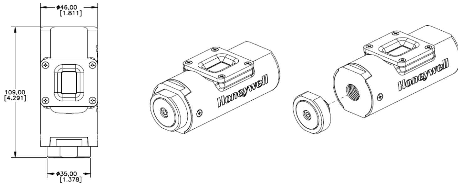
Figure 6– Magnetic mount
