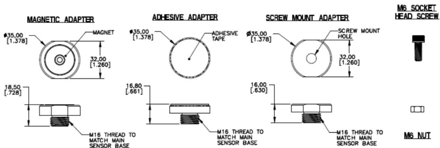
Figure 4– Adapters
