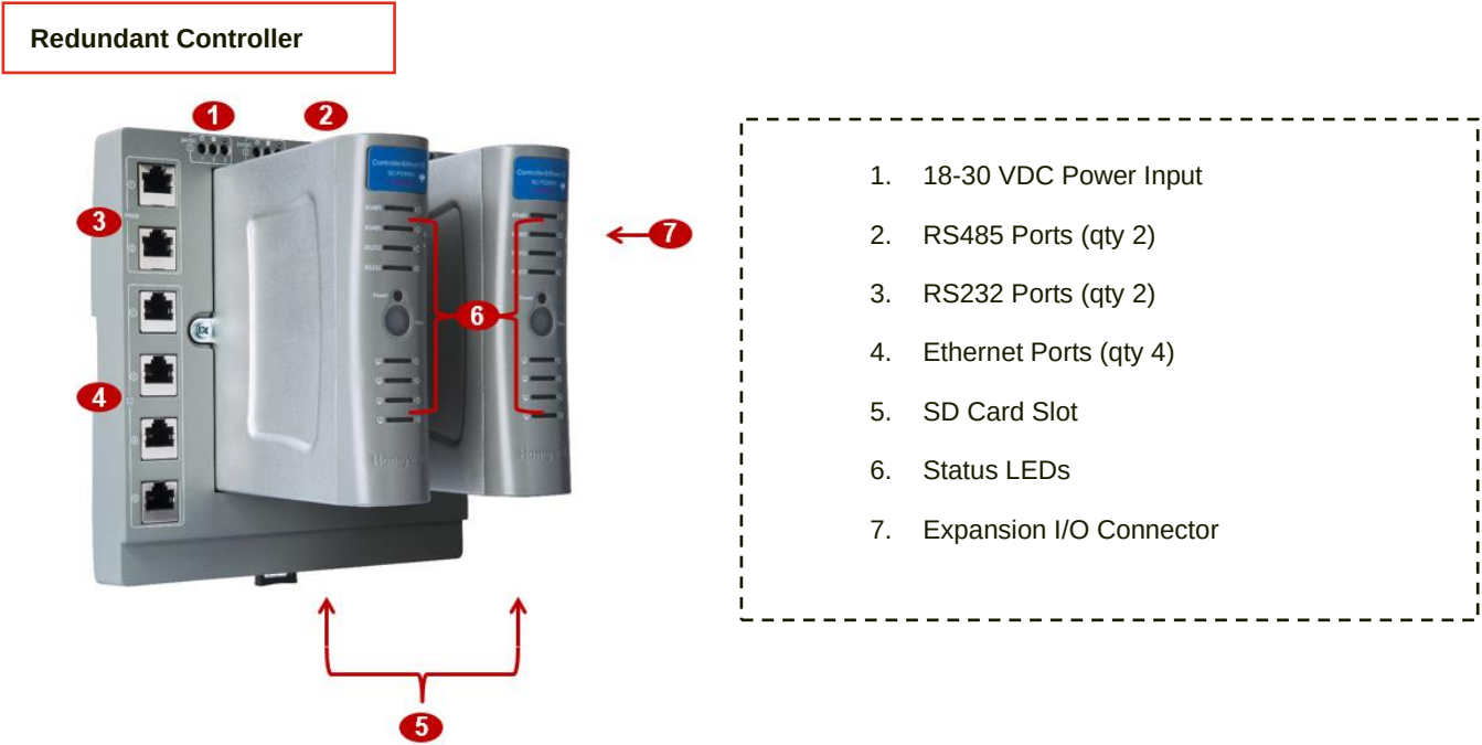
Figure 3 –Redundant Controller Hardware Summary
