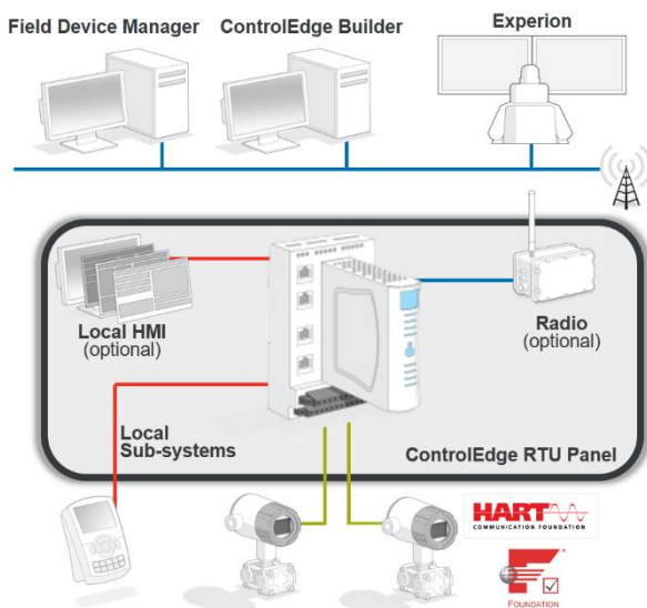
Figure 1 – Sample RTU System Architecture
