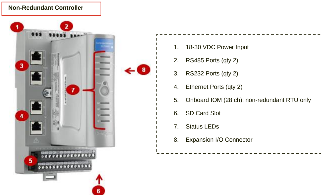
Figure 2 – Non Redundant Controller Hardware Summary
