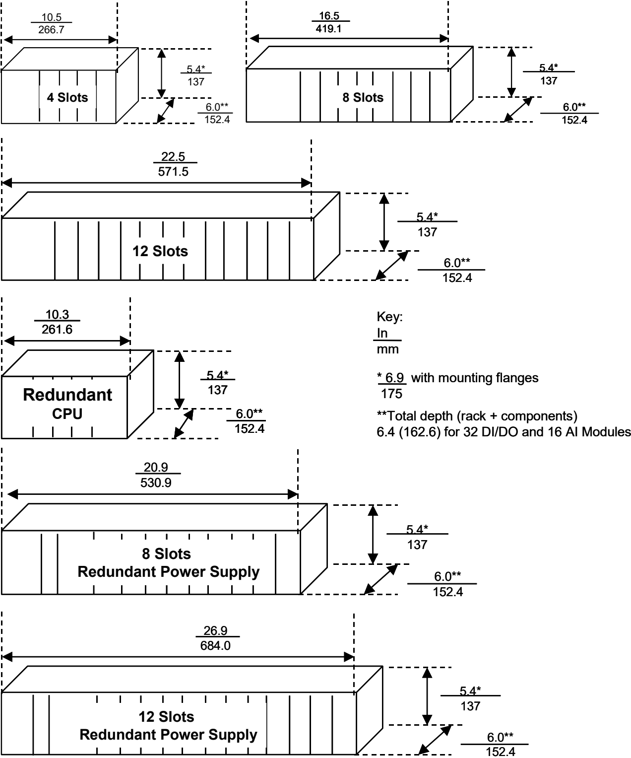
Figure 11 - ControlEdge HC900 Controller Dimensions
